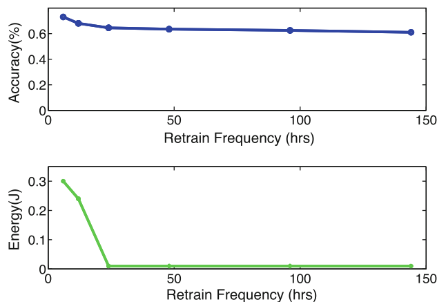
Fig. 8 Trade-off between client energy and classifier accuracy if classifiers are re-trained frequently
